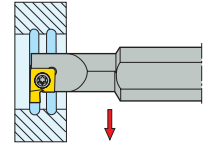
SNR/L KAPR = 90,0 °
