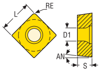
SCGW
