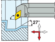
PDUNR/L-15 KAPR = 93,0°
